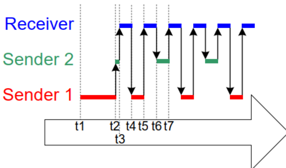
Figure 5.6 The sequence of execution produced by Example 5.2
